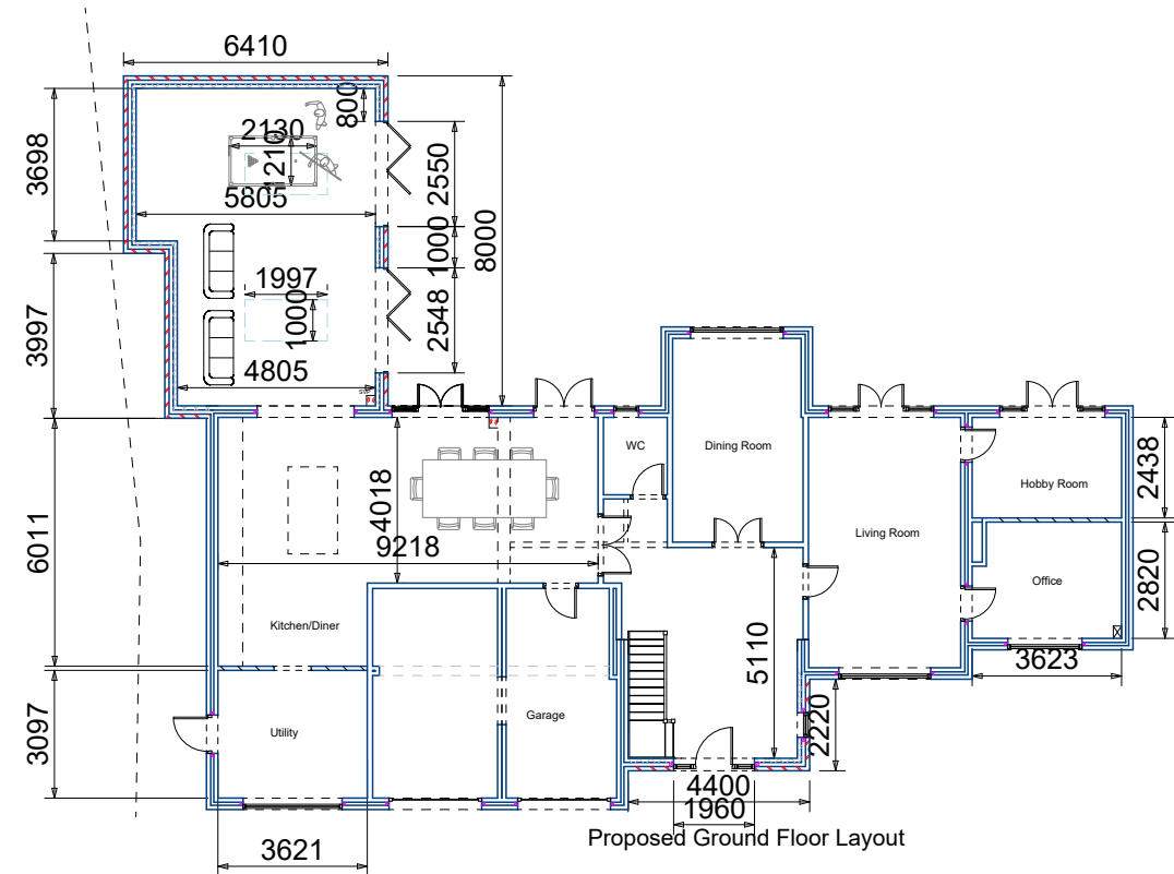
Proposed Ground Floor Layout
