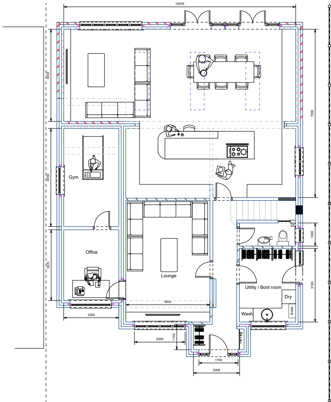
Proposed Ground Floor Layout
