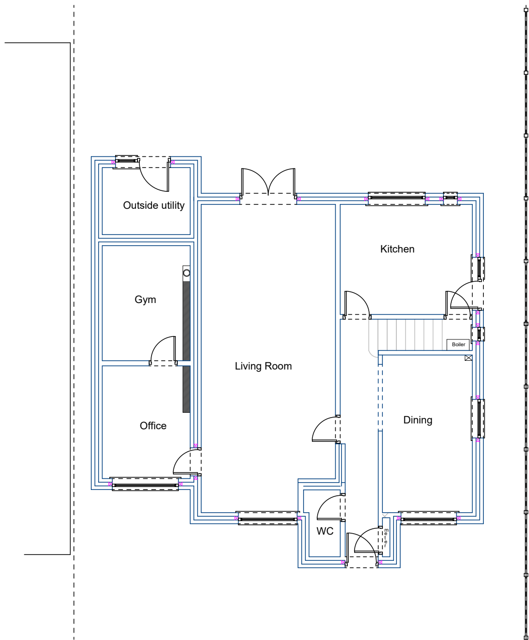
Existing Ground Floor Layout
